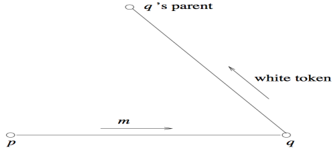
Figure: Node p sends a message m to node q that has already sent a white token to its parent
